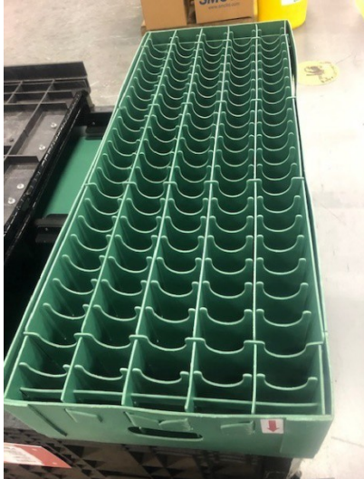
Tray B Dimensions (Blue): 7" tall, 16" Wide, 42" Long (inner compartments 1" x 6")
